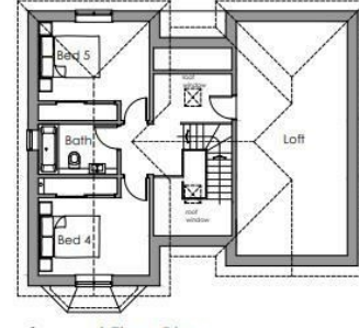
Second Floor Plan ftl=63.825m
