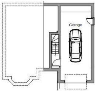
Lower Ground Floor Plan garage fsl = 55.950m
