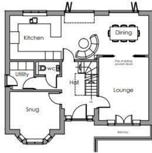
Upper Ground Floor Plan ftl 58.500m
