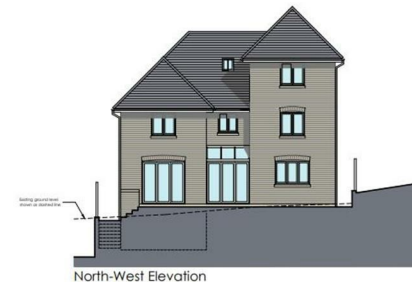
North-West Elevation
